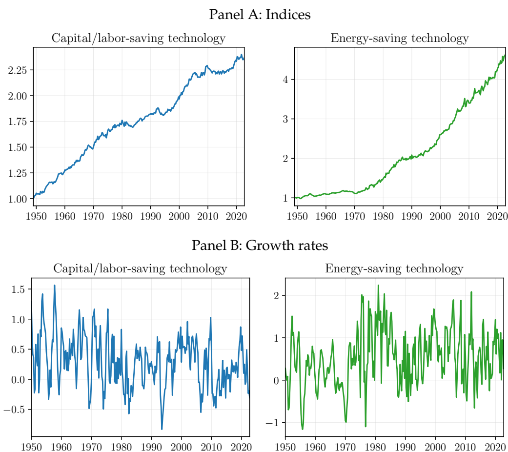
Figure 2: Input-saving technologies
