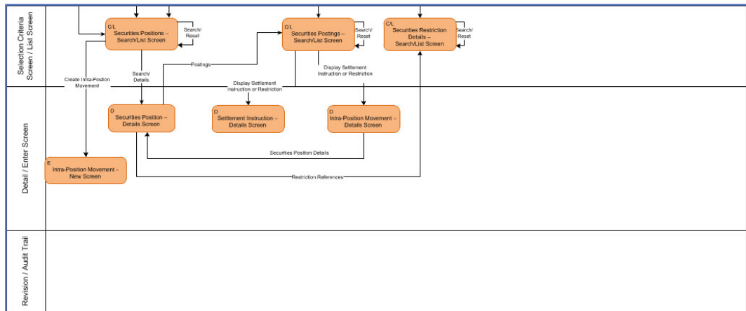
Illustration 315: Screen interrelation
