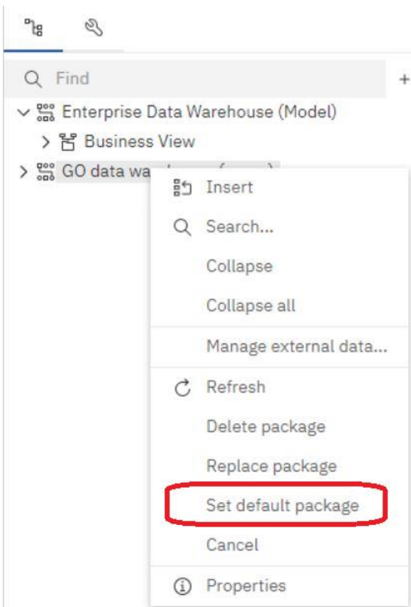
Figure 505 - Adding data - Add a source - Right click item - Set default package
