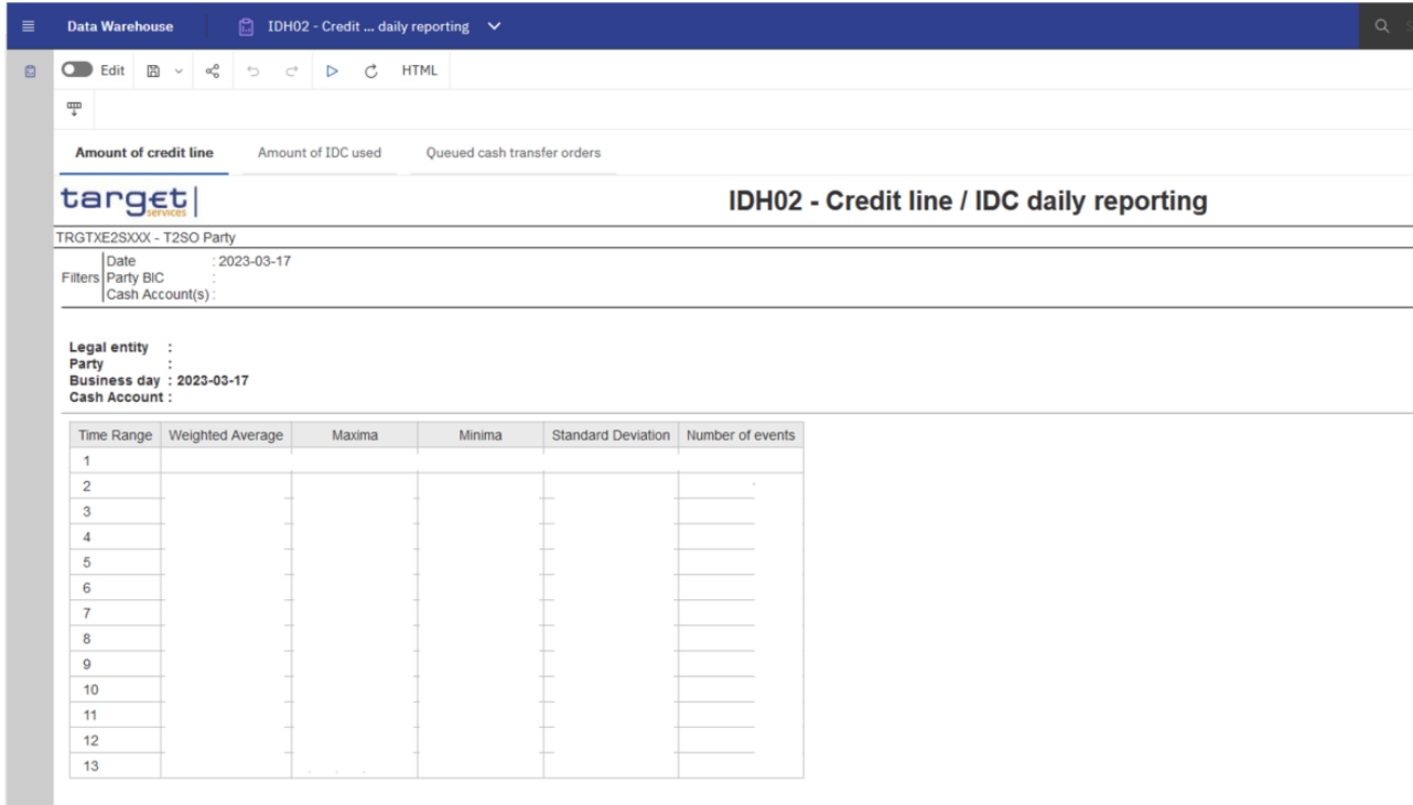
Figure 570 - IDH02 Results screen (1) for credit line amounts (CR-154)
