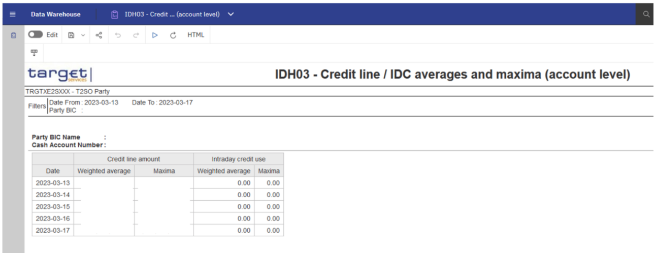
Figure 574 - IDH03 credit line amount and IDC use {CR-154}
