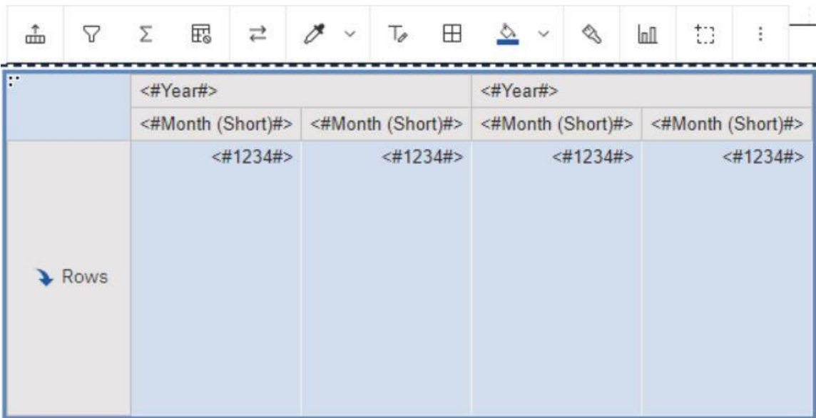
Figure 522 - Create a Single-Edge crosstab
