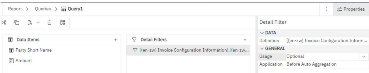
Figure 547 - Create a Prompt Directly in a Report Page
