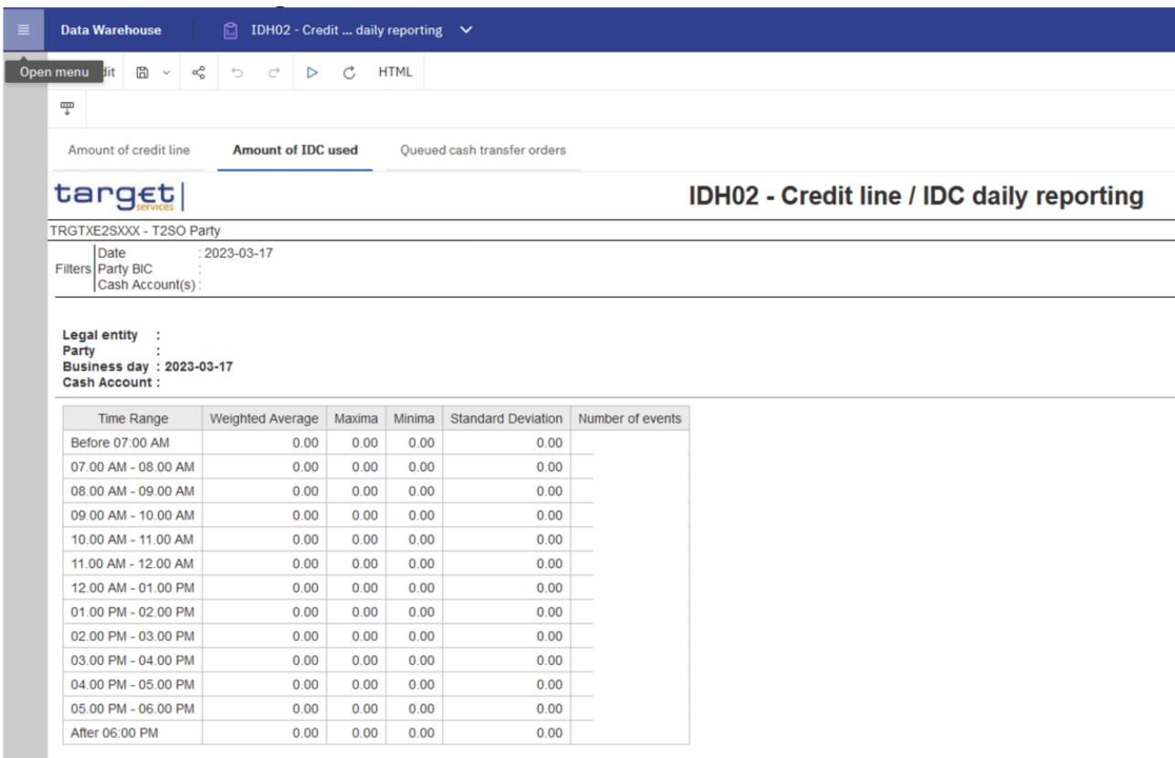
Figure 571 - IDH02 Results screen (2) for intraday credit amount used{CR-154}
