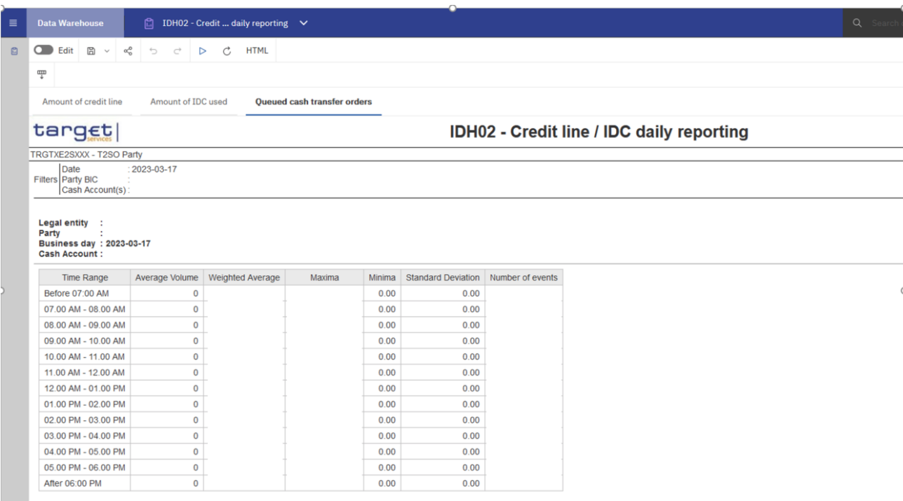
Figure 572 - IDH02 Results screen (3) for queued cash transfer orders{CR-154}
