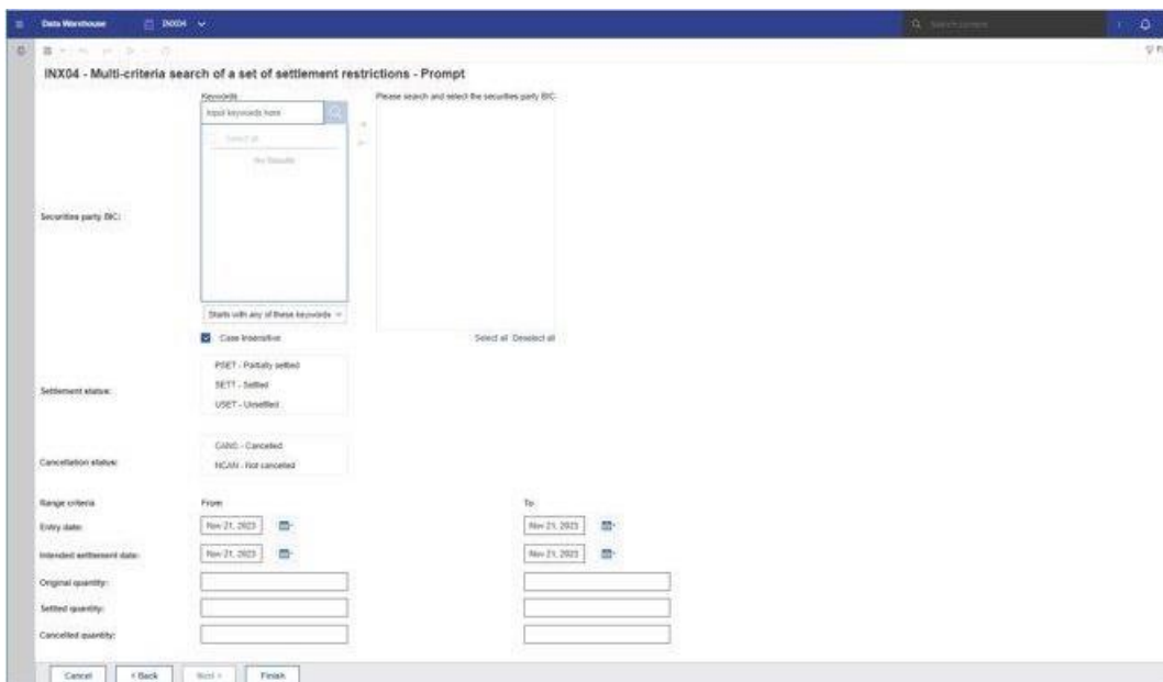
Figure 398 - INX04 prompt screen 2 (CSD User login) {Split book approach, CR-833}
