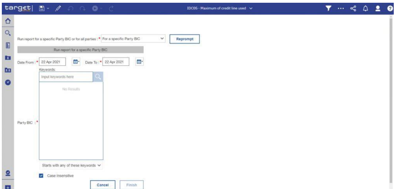
Figure 567 - IDH05 prompt screen with specific party BIC selection {CR-143}
