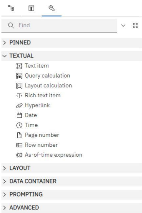
Figure 466 - Report objects - Mostly Used Objects - Textual
