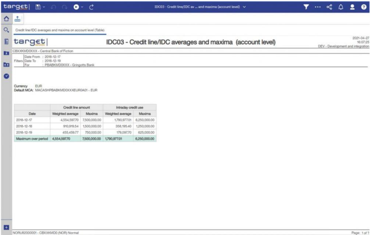
Figure 566 - IDH03 credit line amount and IDC use {CR-143}
