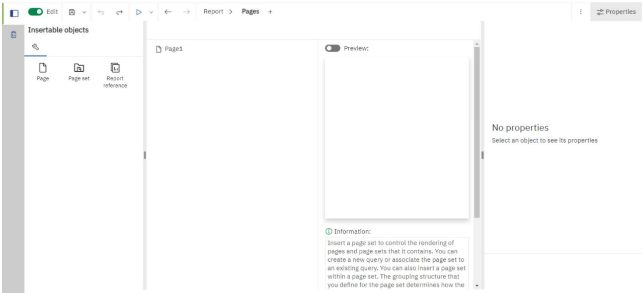
Figure 448 - Pages pane
