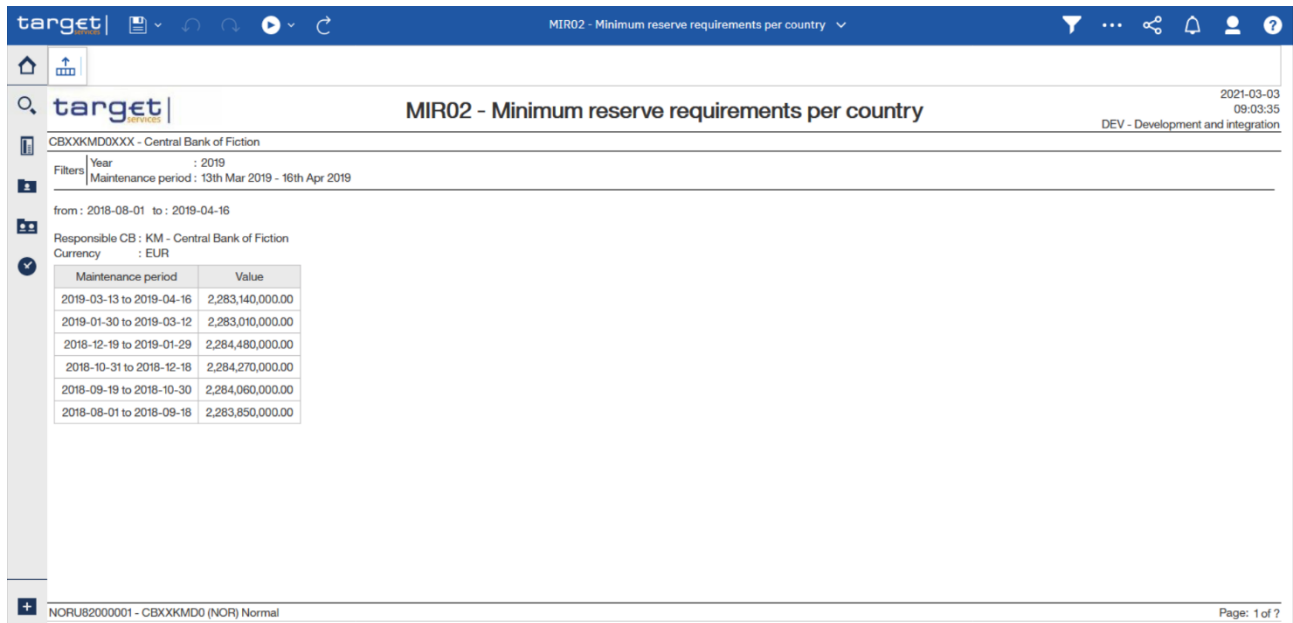
Figure 278 - MIR02 output
