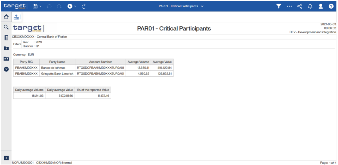
Figure 284 - PAR01 output (1)
