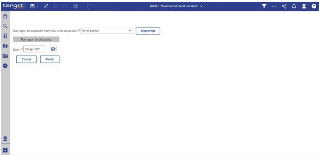
Figure 568 - IDH05 prompt screen with multiple party selection {CR-143}
