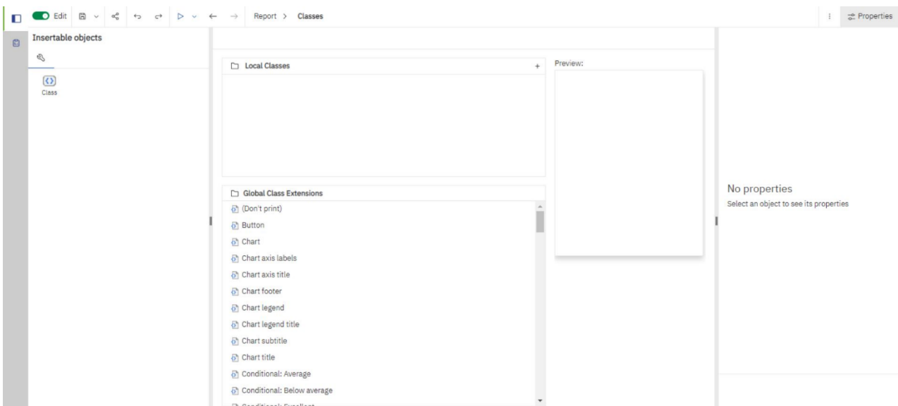
Figure 450 - Classes pane
