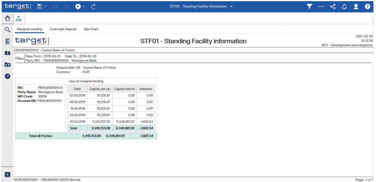
Figure 302 - STF01 output (1)
