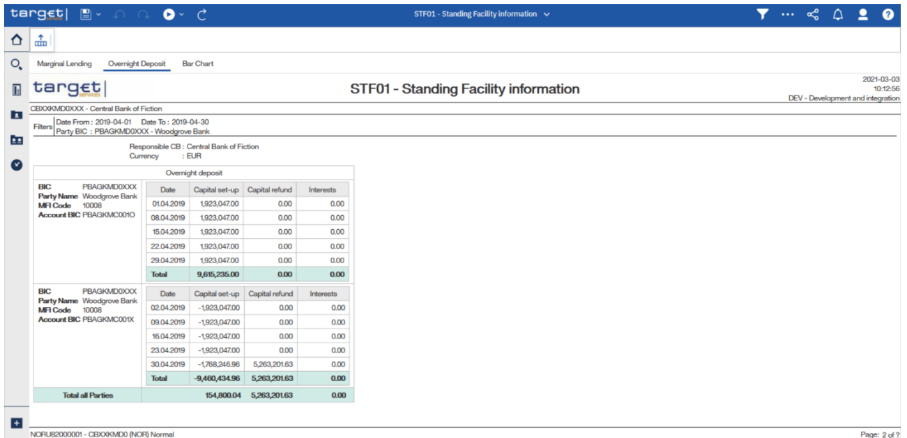
Figure 303 - STF01 output (2)
