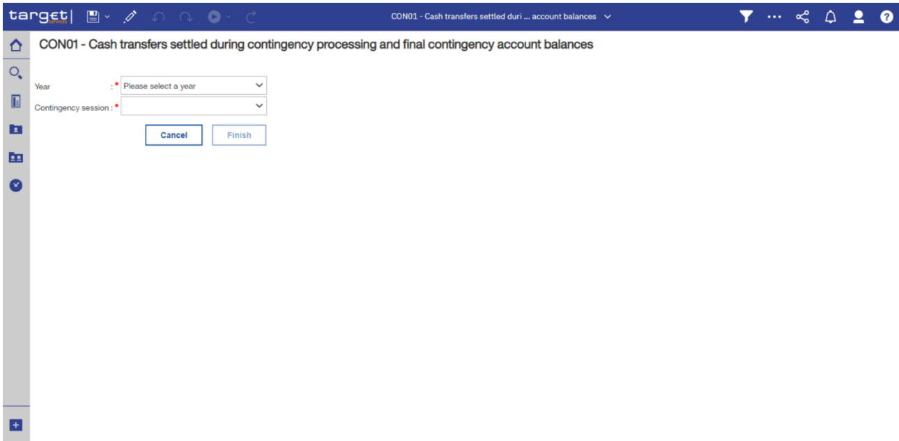
Figure 231 - CON1 prompt
