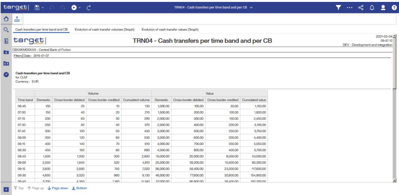
Figure 330 - TRN04 output (1)
