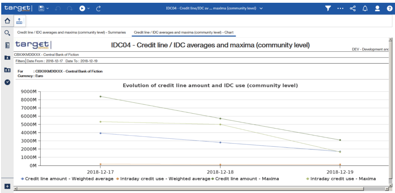
Figure 258 - IDC04 output (2)
