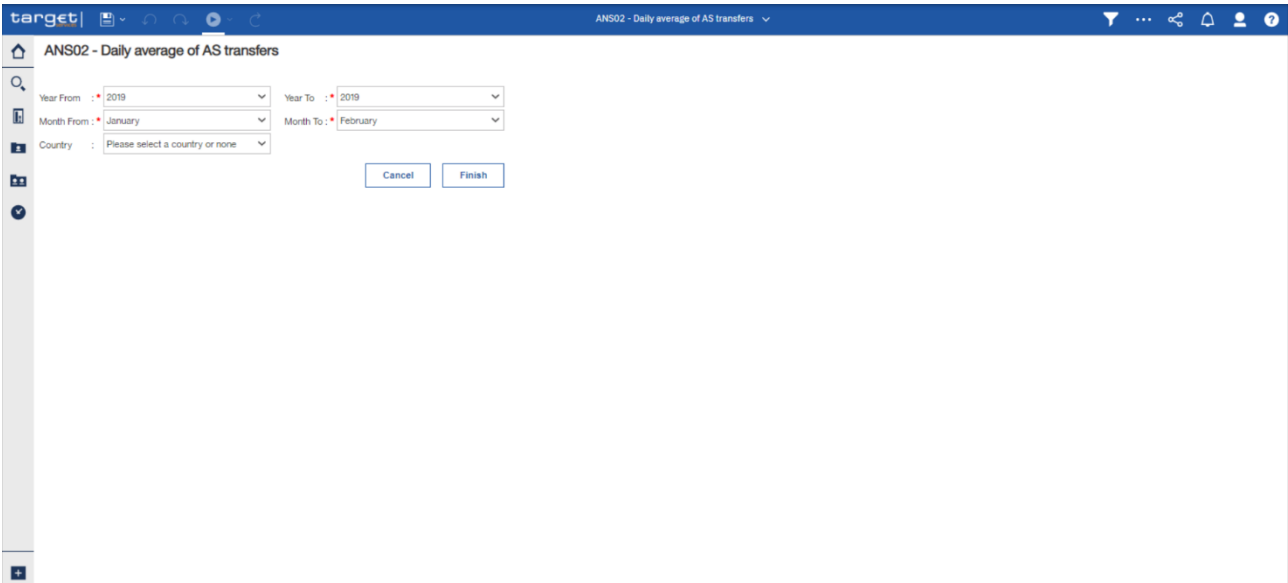
Figure 180 - ANS02 Prompt
