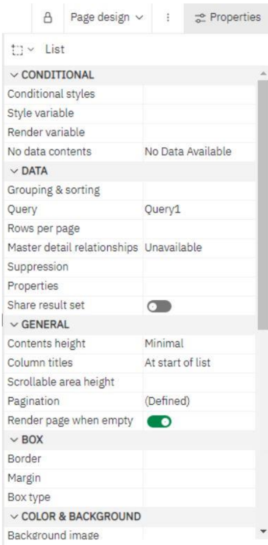
Figure 502 - Set list properties
