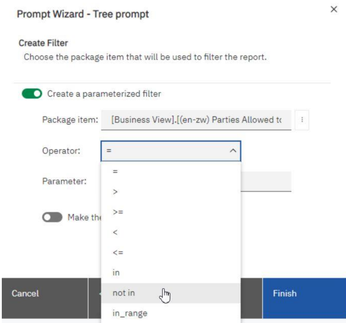
Figure 542 - Control the data that appears in a tree prompt - Prompt Wizard - Operator
