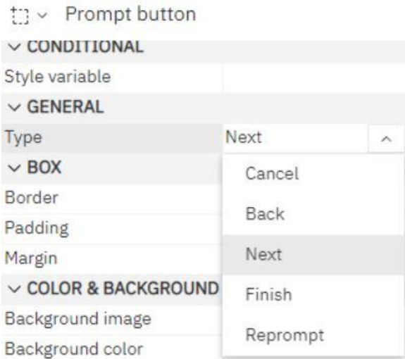
Figure 558 - Modifying prompts - Add prompt buttons - Prompt button properties - General - Type
