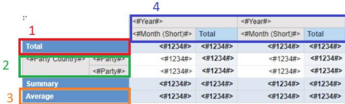
Figure 512 - Crosstab nodes and Crosstab nodes members (2)
