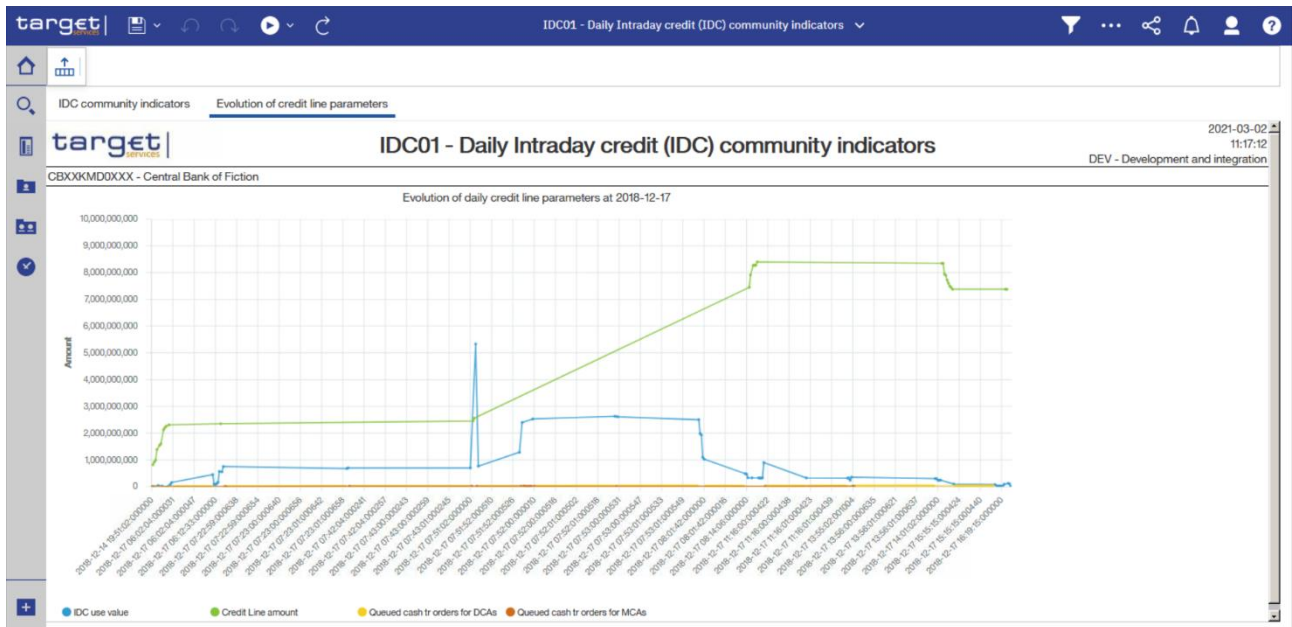
Figure 245 - IDC01 Output (2)
