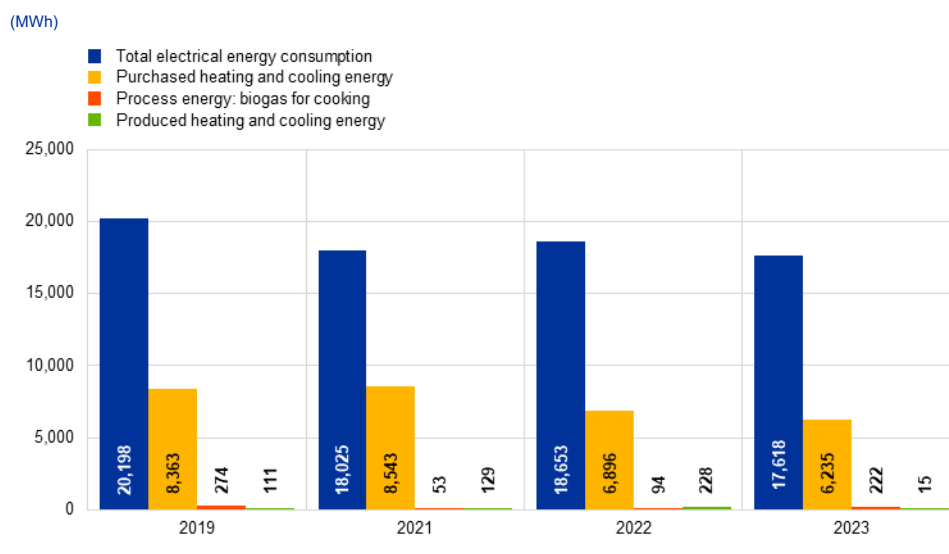
Chart 5 Energy consumption – main building 10
